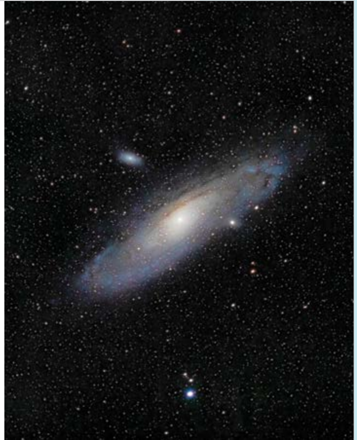
Andromeda Galaxy
